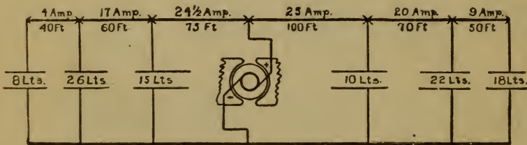
Figure 5 Ordinary lighting circuit.
